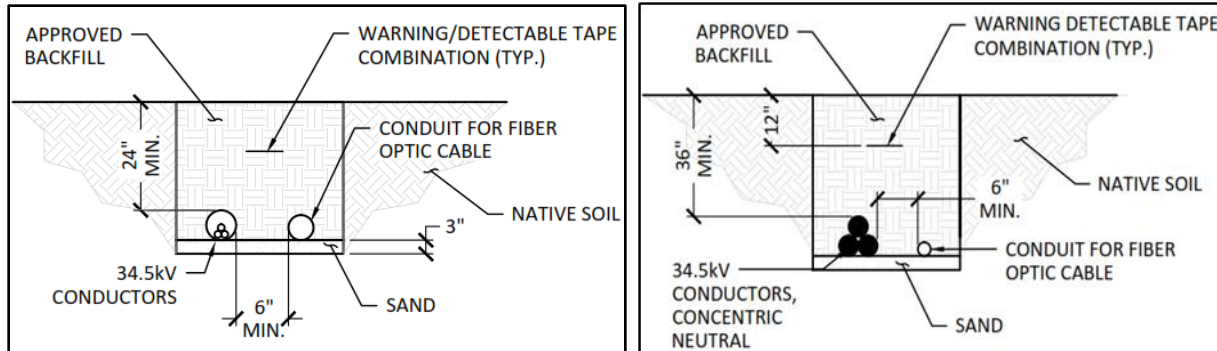
Figure 8-1. Electrical Collection System Trench Design
