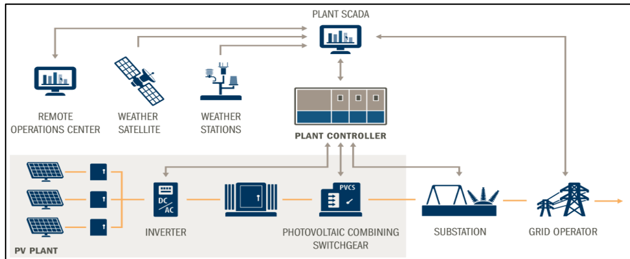
Figure 7-7. Typical SCADA System
