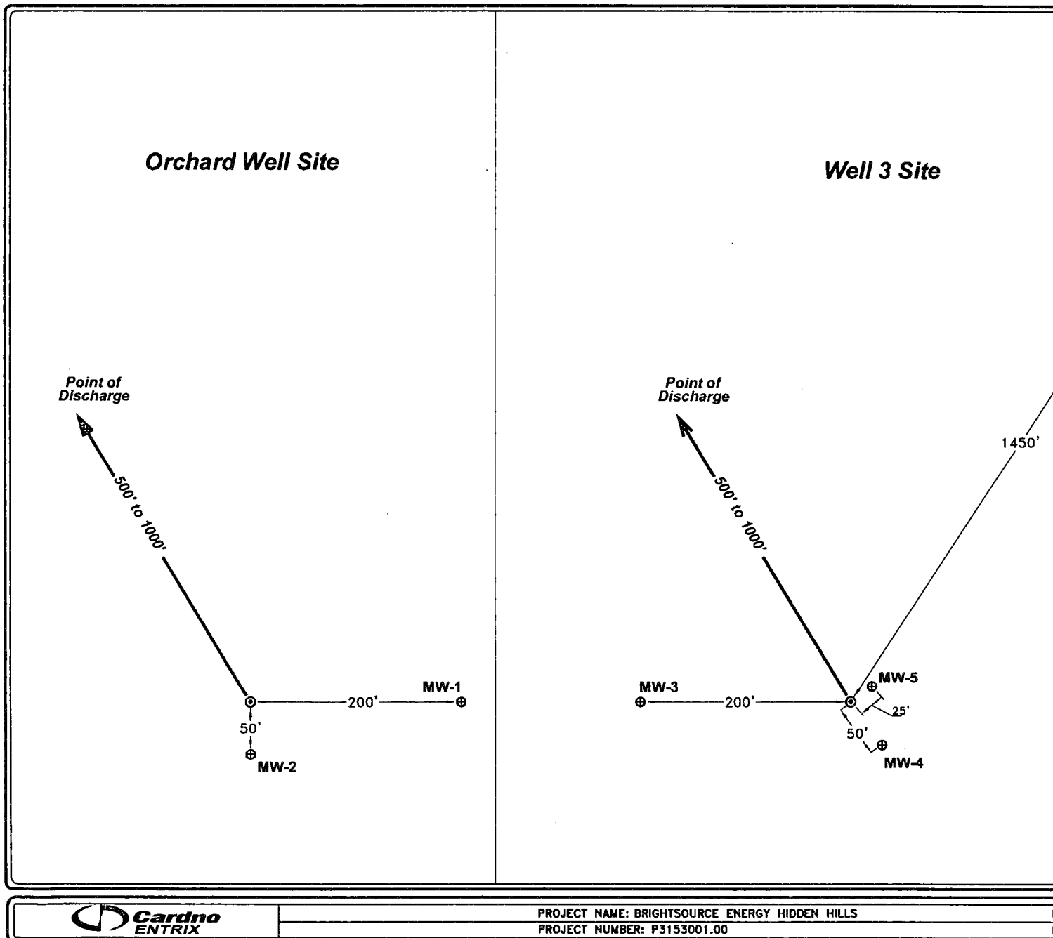
FIGURE 1-2. PROPOSED APT MONITOR WELL LOCATIONS.
