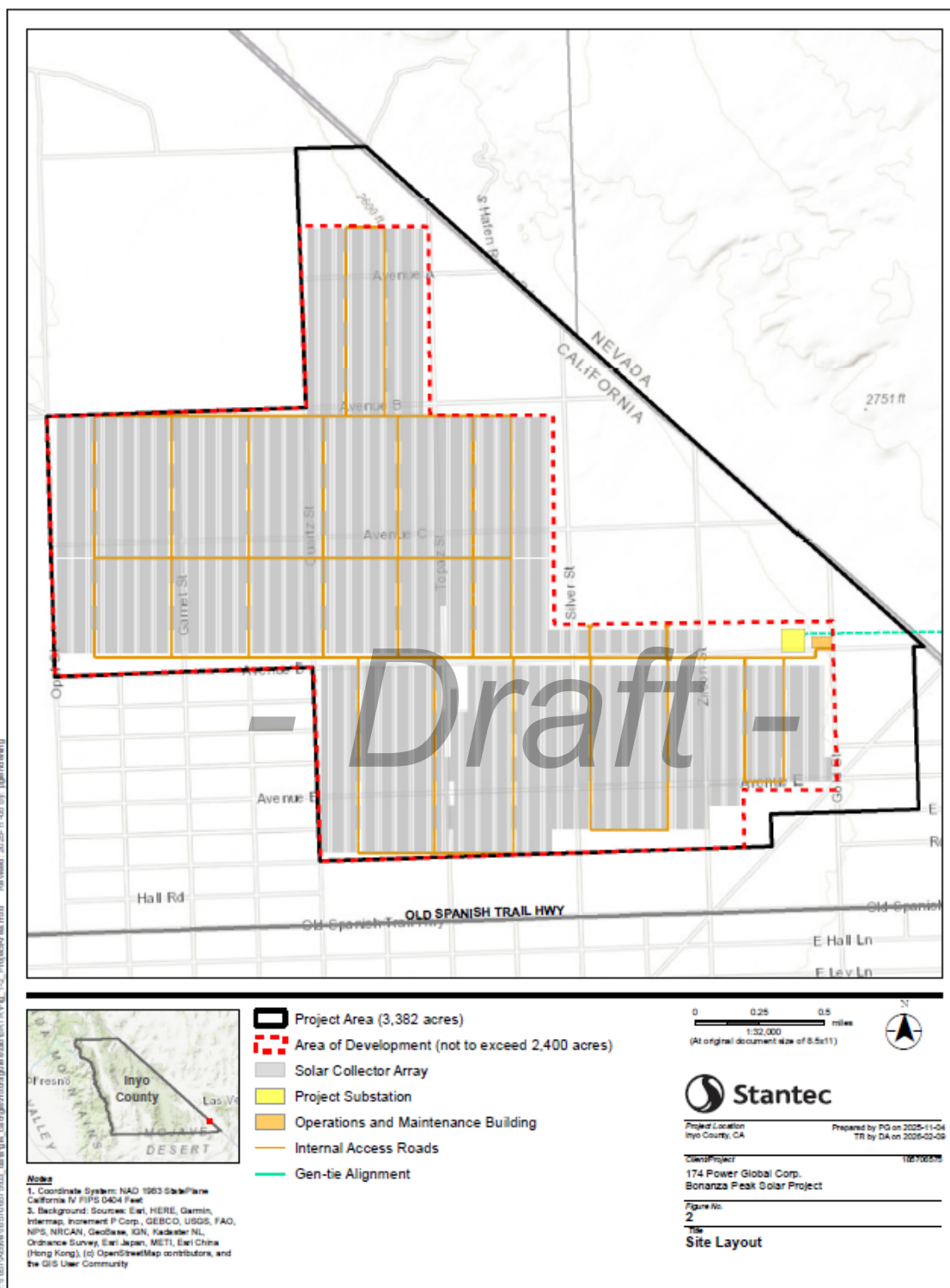
Figure 2. Site Layout
