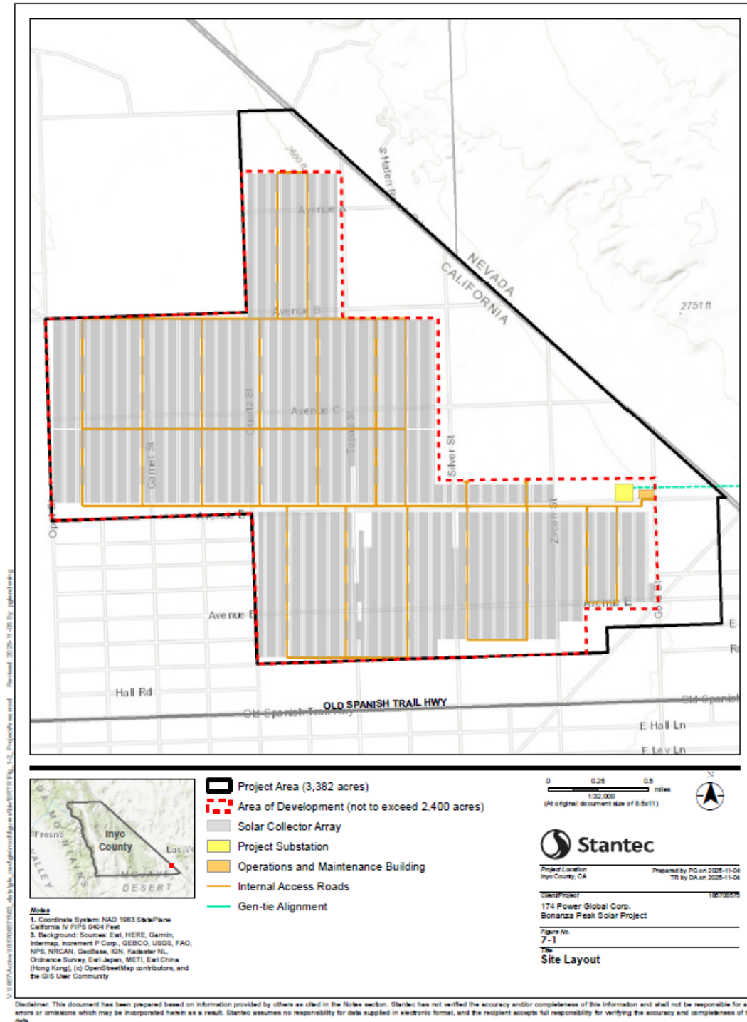
Figure 7-1. Site Layout
